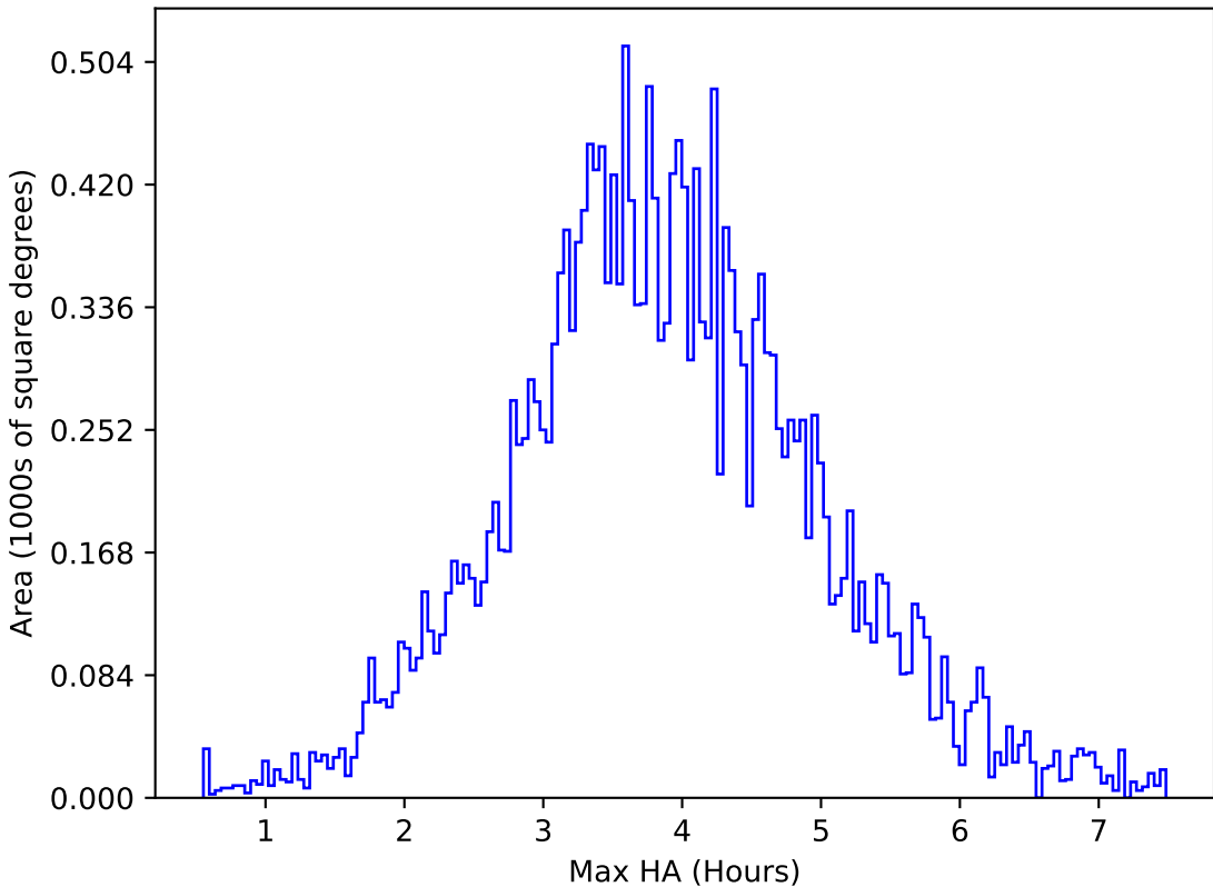
too_elab_heavy_r32_d2_ugrizy_v3.4_10yrs All sky u band: Max HA
