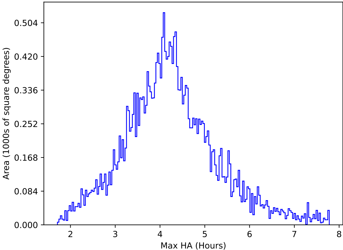
too_elab_heavy_r32_d2_ugrizy_v3.4_10yrs All sky r band: Max HA
