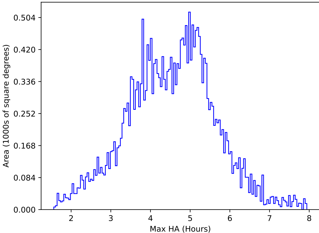
too_elab_heavy_r32_d2_ugrizy_v3.4_10yrs All sky i band: Max HA
