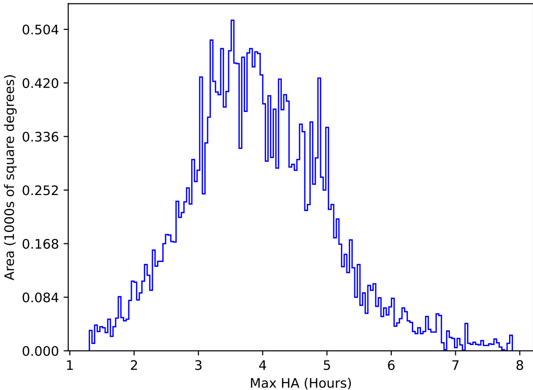
too_elab_heavy_r32_d2_ugrizy_v3.4_10yrs All sky g band: Max HA
