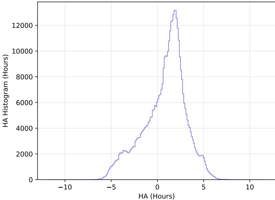
too_elab_heavy_r32_d2_ugrizy_v3.4_10yrs WFD z band: HA Histogram
