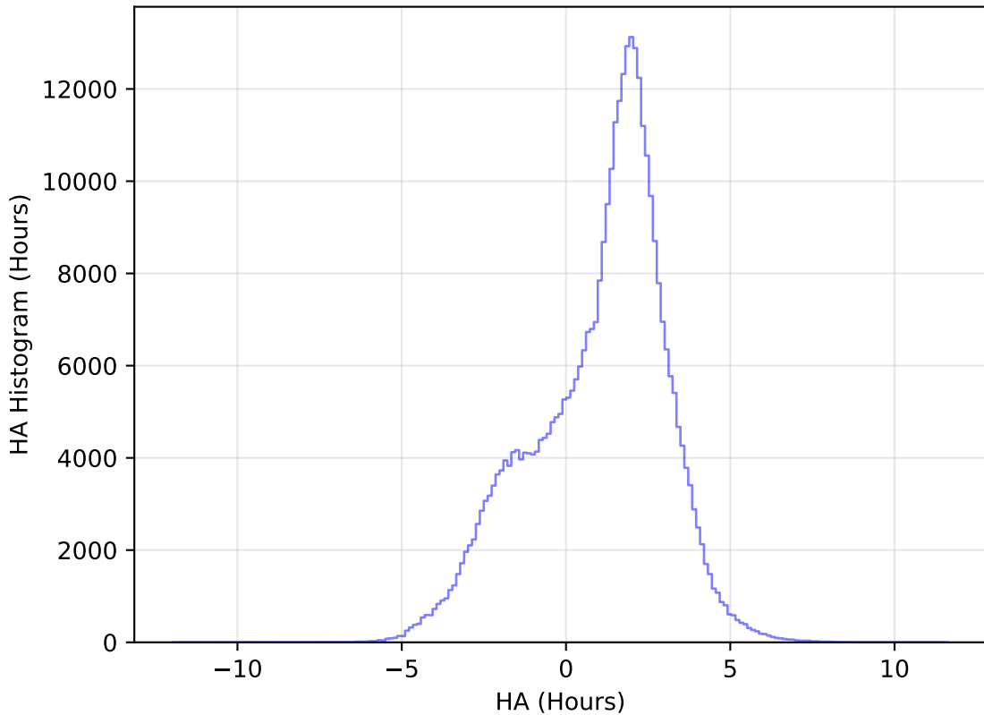
too_elab_heavy_r32_d2_ugrizy_v3.4_10yrs WFD y band: HA Histogram
