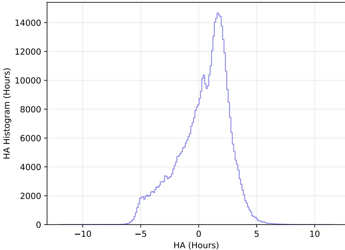
too_elab_heavy_r32_d2_ugrizy_v3.4_10yrs WFD r band: HA Histogram
