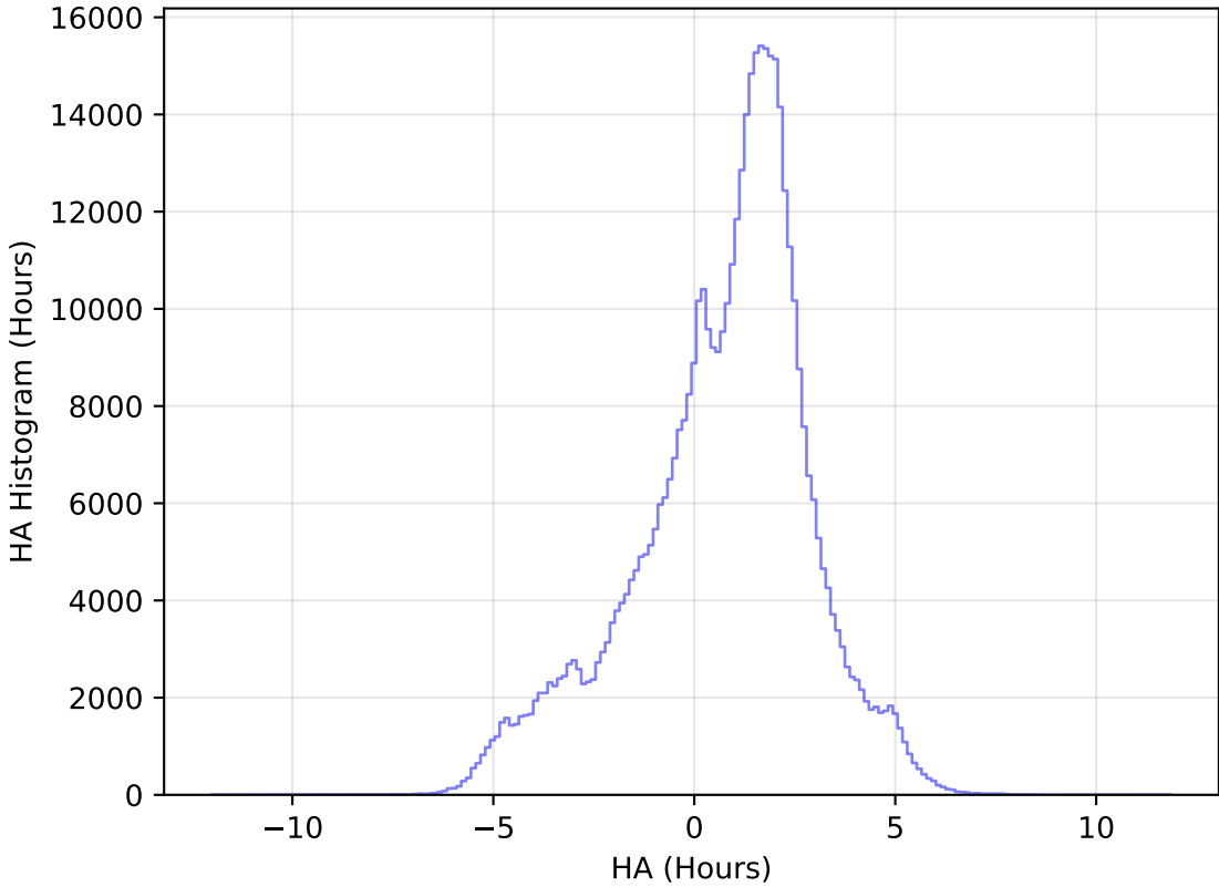
too_elab_heavy_r32_d2_ugrizy_v3.4_10yrs WFD i band: HA Histogram
