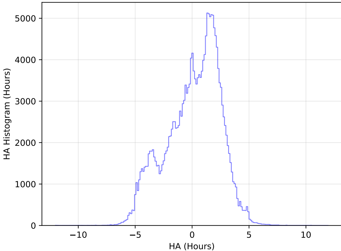
too_elab_heavy_r32_d2_ugrizy_v3.4_10yrs WFD g band: HA Histogram
