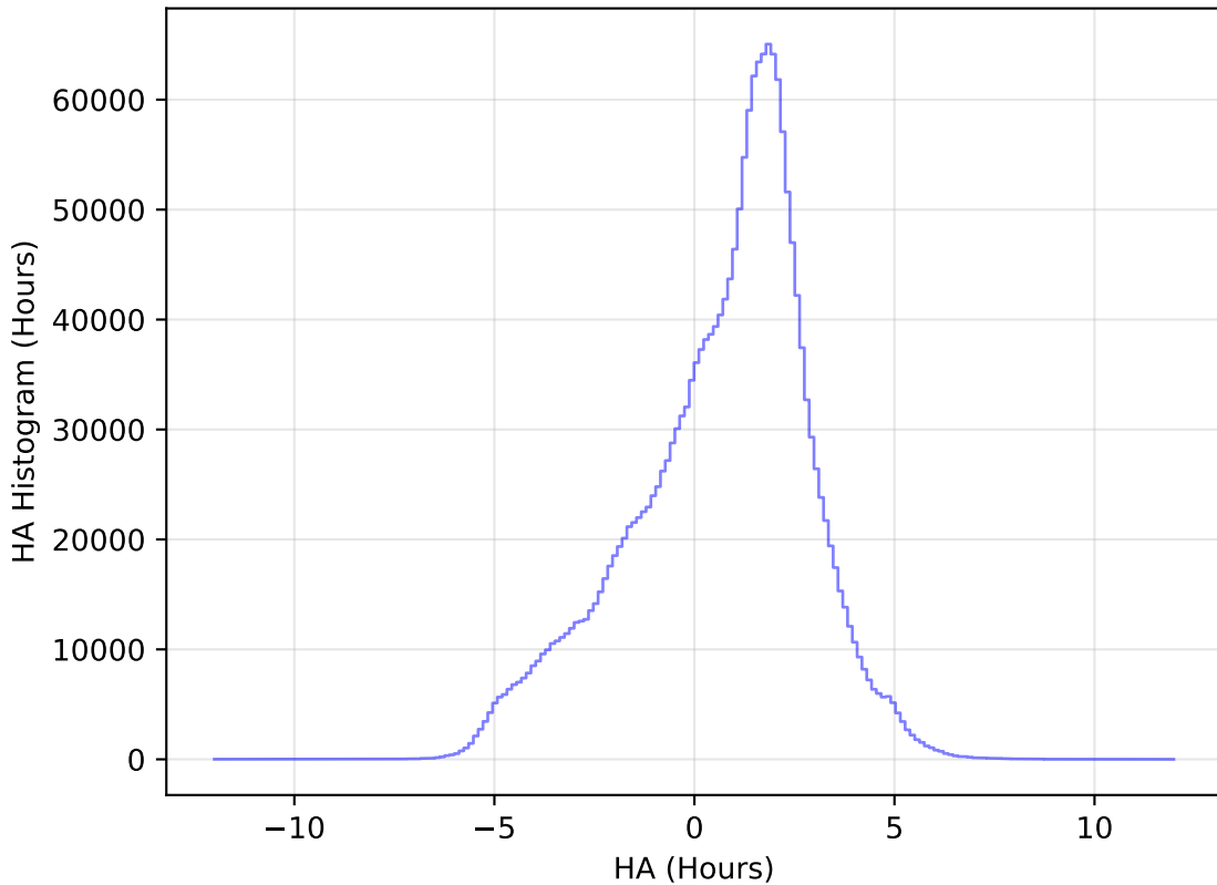
too_elab_heavy_r32_d2_ugrizy_v3.4_10yrs WFD all bands: HA Histogram
