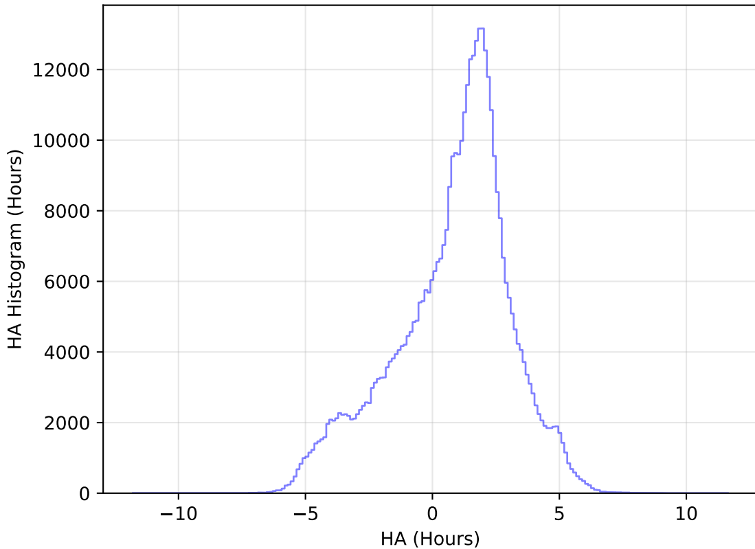
too_elab_heavy_r32_d2_ugrizy_v3.4_10yrs All sky z band: HA Histogram
