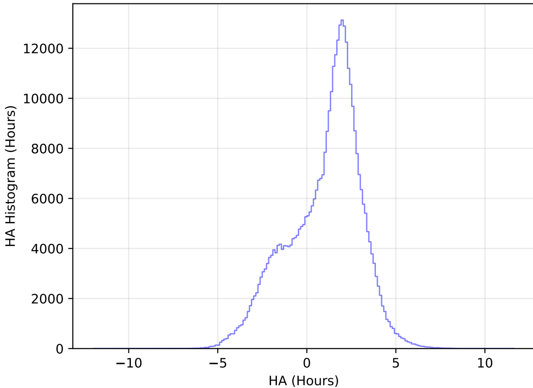
too_elab_heavy_r32_d2_ugrizy_v3.4_10yrs All sky y band: HA Histogram
