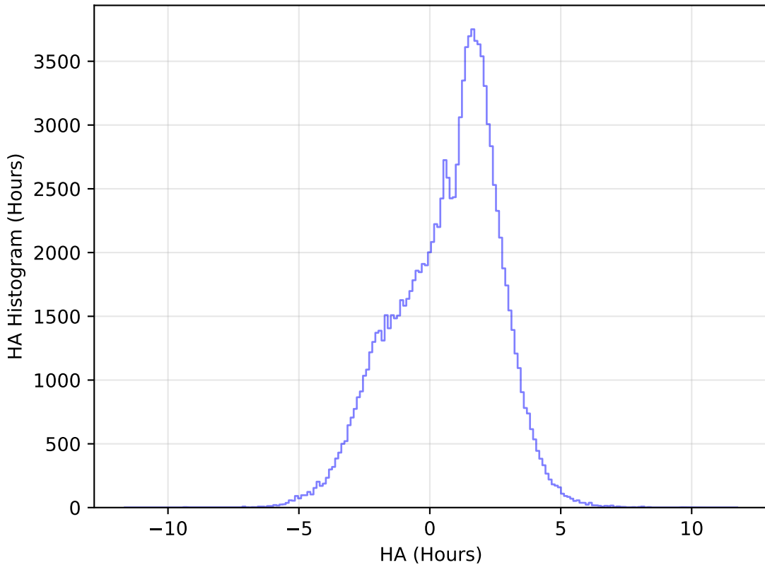
too_elab_heavy_r32_d2_ugrizy_v3.4_10yrs All sky u band: HA Histogram
