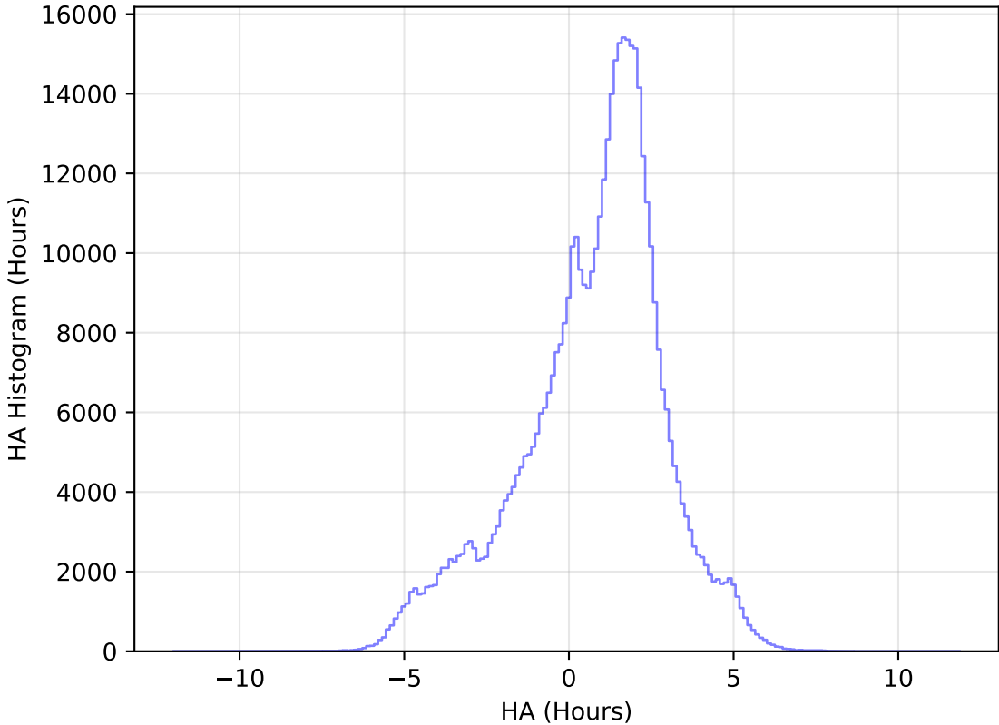
too_elab_heavy_r32_d2_ugrizy_v3.4_10yrs All sky i band: HA Histogram
