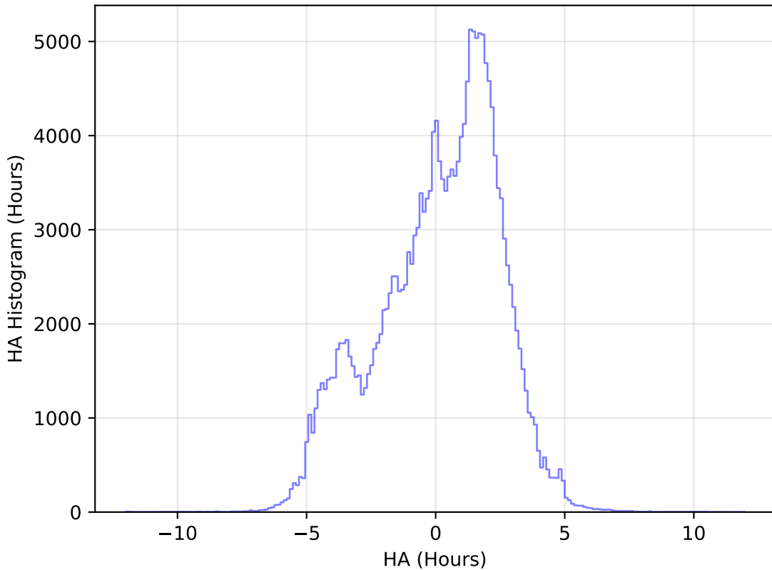
too_elab_heavy_r32_d2_ugrizy_v3.4_10yrs All sky g band: HA Histogram
