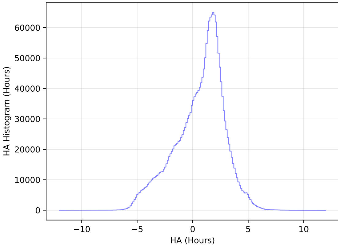
too_elab_heavy_r32_d2_ugrizy_v3.4_10yrs All sky all bands: HA Histogram
