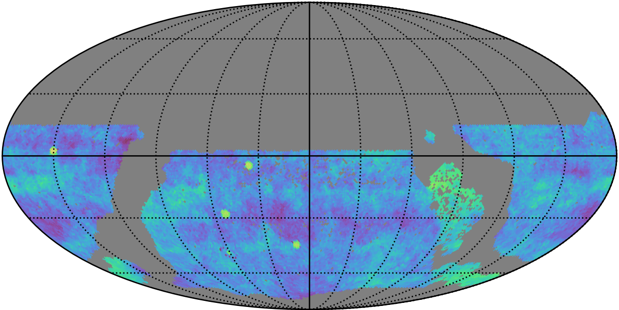
too_elab_heavy_r32_d2_ugrizy_v3.4_10yrs gri WFD: Fraction of visits in pairs (20-90 min)
