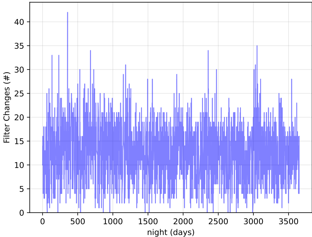
too_elab_heavy_r32_d2_ugrizyv3.4_10yrs Per Night: Filter Changes
