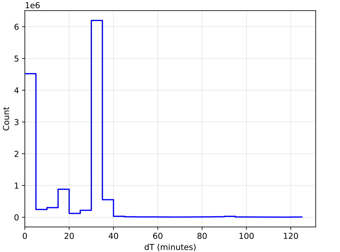
too_elab_heavy_r32_d2_ugrizy_v3.4_10yrs All sky: DeltaT Histogram
