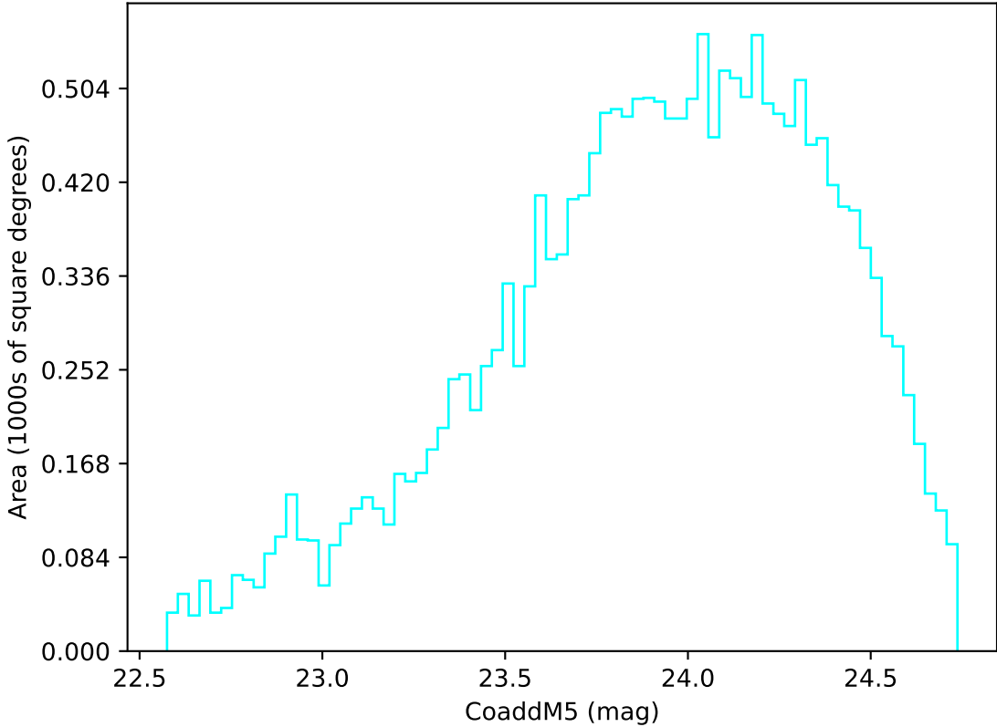
too_elab_heavy_r32_d2_ugrizy_v3.4_10yrs Yr 3-4 u band: CoaddM5
