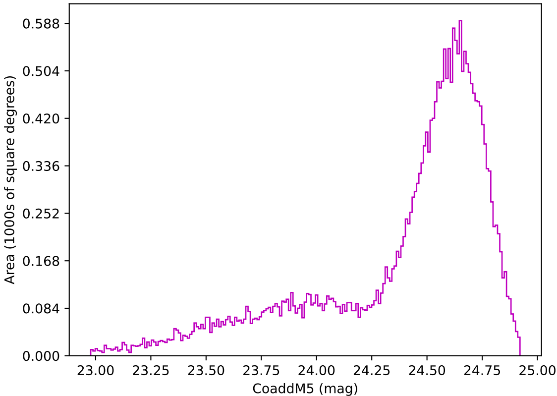
too_elab_heavy_r32_d2_ugrizy_v3.4_10yrs Yr 1 z band: CoaddM5
