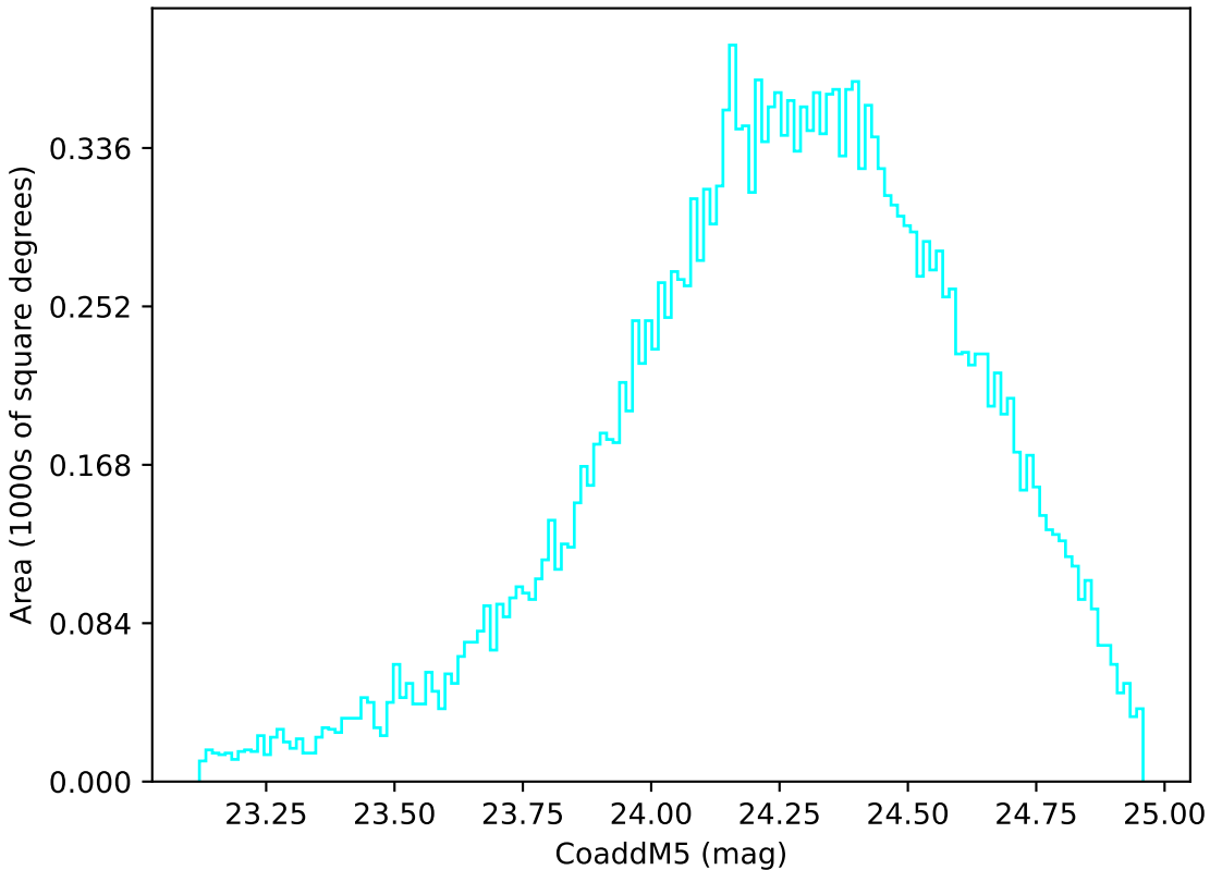
too_elab_heavy_r32_d2_ugrizy_v3.4_10yrs Yr 1 u band: CoaddM5
