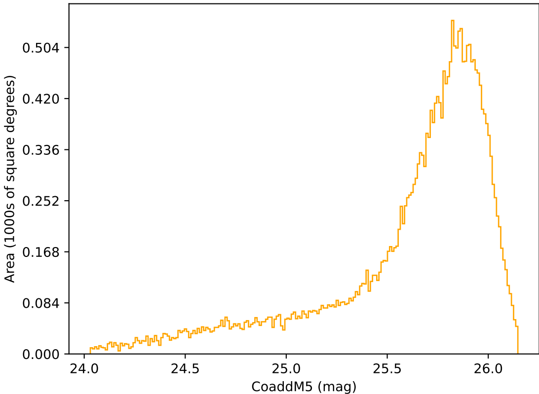
too_elab_heavy_r32_d2_ugrizy_v3.4_10yrs Yr 1 r band: CoaddM5
