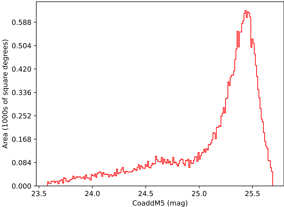
too_elab_heavy_r32_d2_ugrizy_v3.4_10yrs Yr 1 i band: CoaddM5
