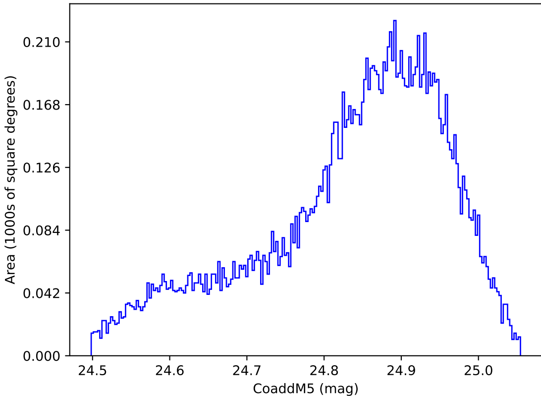
too_elab_heavy_r32_d2_ugrizy_v3.4_10yrs WFD y band: CoaddM5
