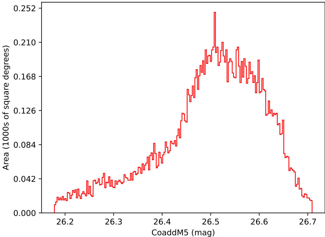
too_elab_heavy_r32_d2_ugrizy_v3.4_10yrs WFD i band: CoaddM5
