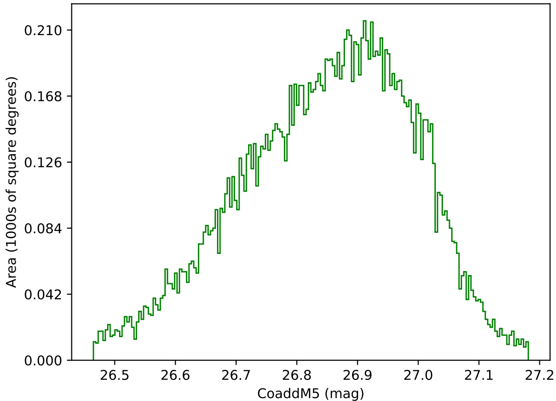
too_elab_heavy_r32_d2_ugrizy_v3.4_10yrs WFD g band: CoaddM5
