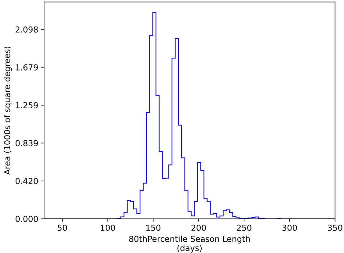
too_elab_heavy_r32_d2_ugrizy_v3.4_10yrs WFD y band: 80thPercentile Season Length
