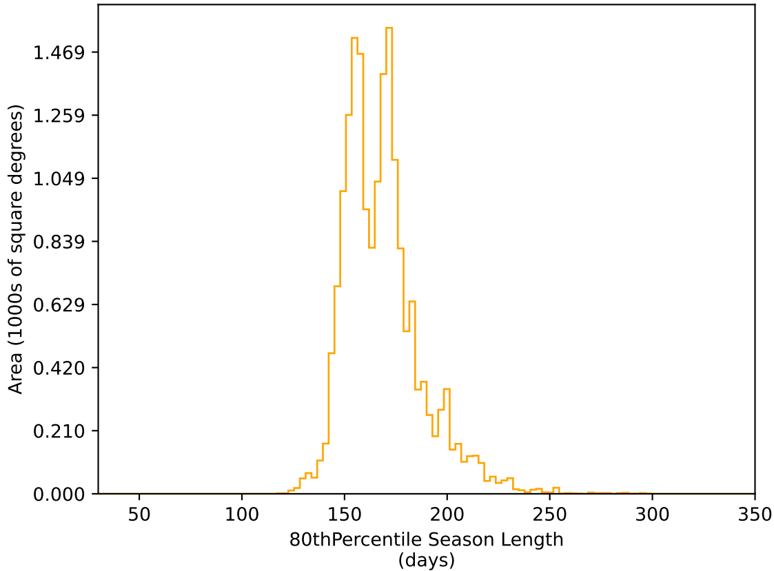
too_elab_heavy_r32_d2_ugrizy_v3.4_10yrs WFD r band: 80thPercentile Season Length
