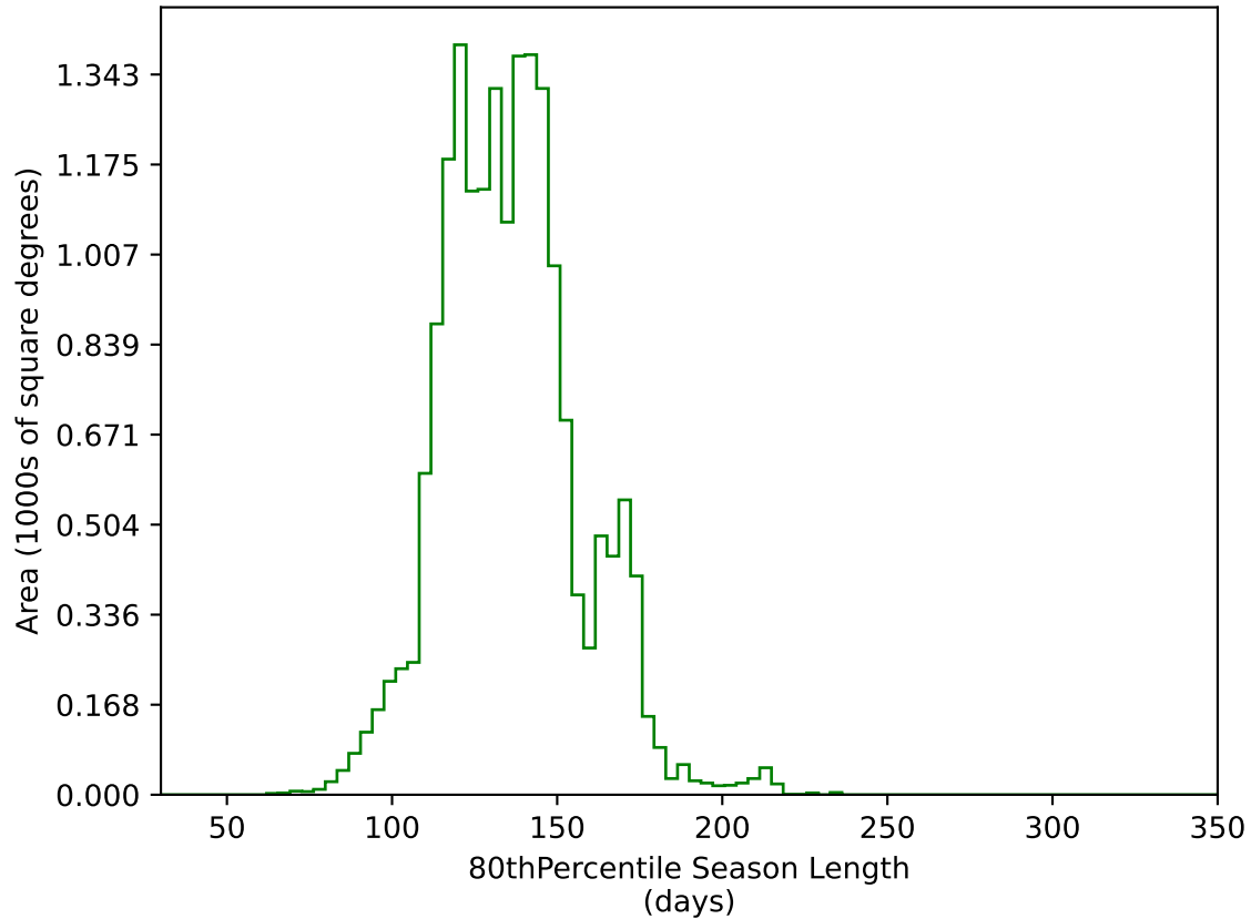
too_elab_heavy_r32_d2_ugrizy_v3.4_10yrs WFD g band: 80thPercentile Season Length
