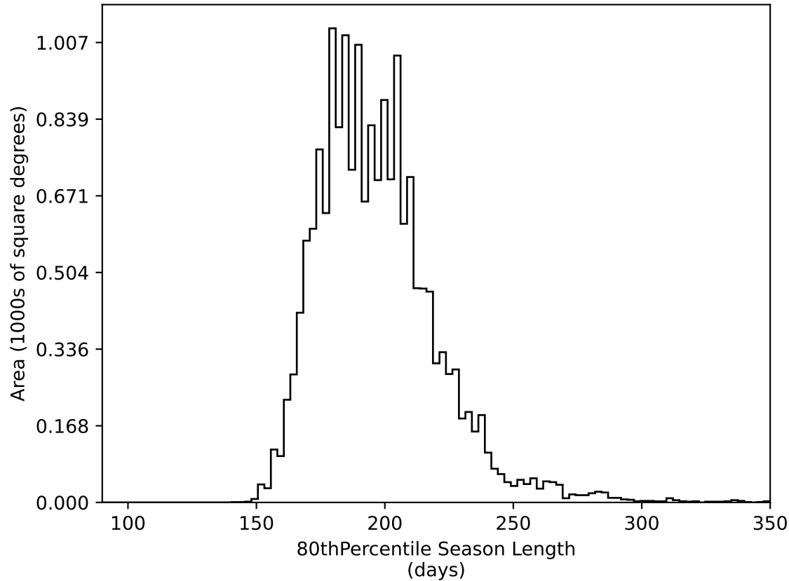
too_elab_heavy_r32_d2_ugrizy_v3.4_10yrs WFD all bands: 80thPercentile Season Length
