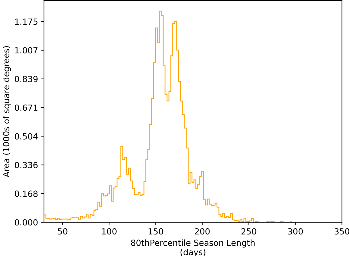
too_elab_heavy_r32_d2_ugrizy_v3.4_10yrs All sky r band: 80thPercentile Season Length
