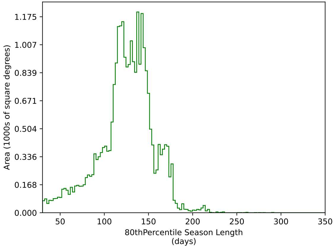
too_elab_heavy_r32_d2_ugrizy_v3.4_10yrs All sky g band: 80thPercentile Season Length
