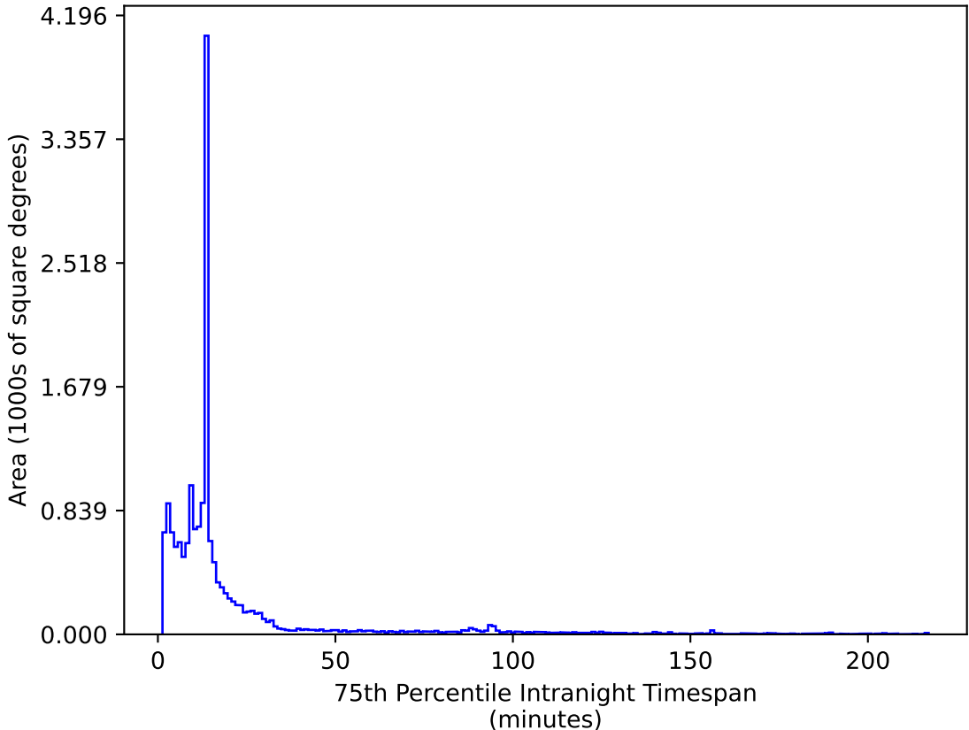
too_elab_heavy_r32_d2_ugrizy_v3.4_10yrs WFD z band: 75th Percentile Intranight Timespan
