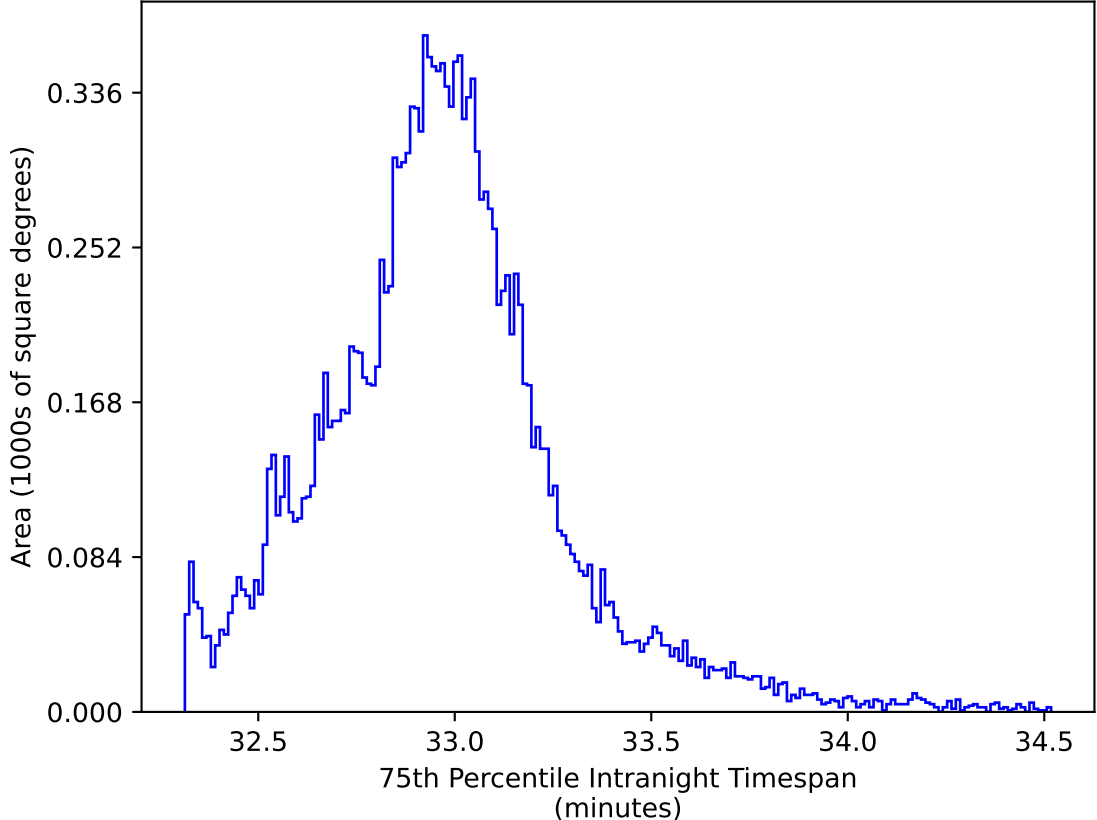
too_elab_heavy_r32_d2_ugrizy_v3.4_10yrs WFD y band: 75th Percentile Intranight Timespan
