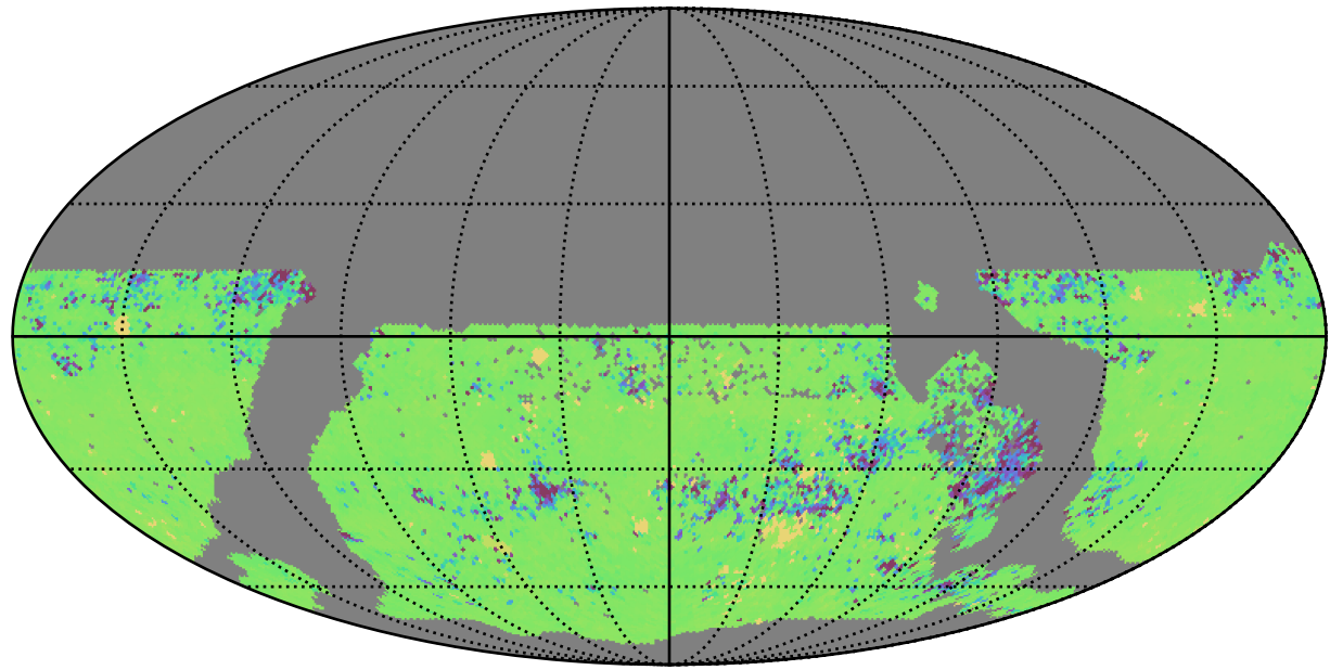
too_elab_heavy_r32_d2_ugrizy_v3.4_10yrs WFD ug bands: 75th Percentile Intranight Timespan
