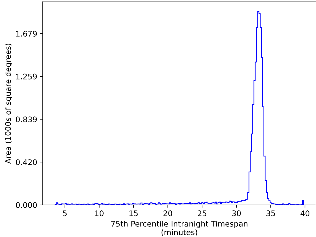
too_elab_heavy_r32_d2_ugrizy_v3.4_10yrs WFD ug bands: 75th Percentile Intranight Timespan
