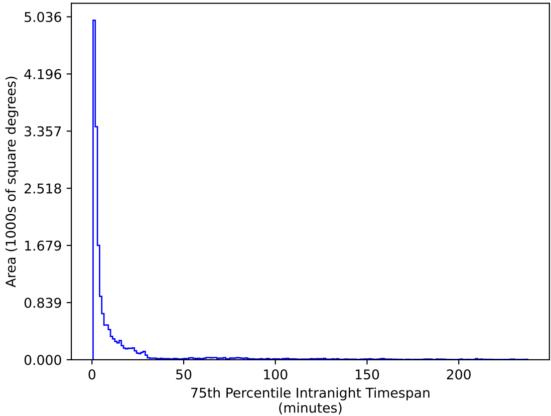
too_elab_heavy_r32_d2_ugrizy_v3.4_10yrs WFD u band: 75th Percentile Intranight Timespan
