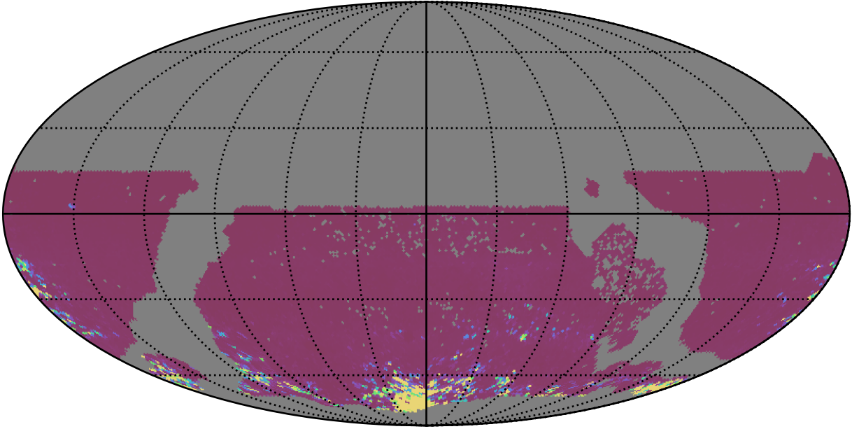
too_elab_heavy_r32_d2_ugrizy_v3.4_10yrs WFD ri bands: 75th Percentile Intranight Timespan
