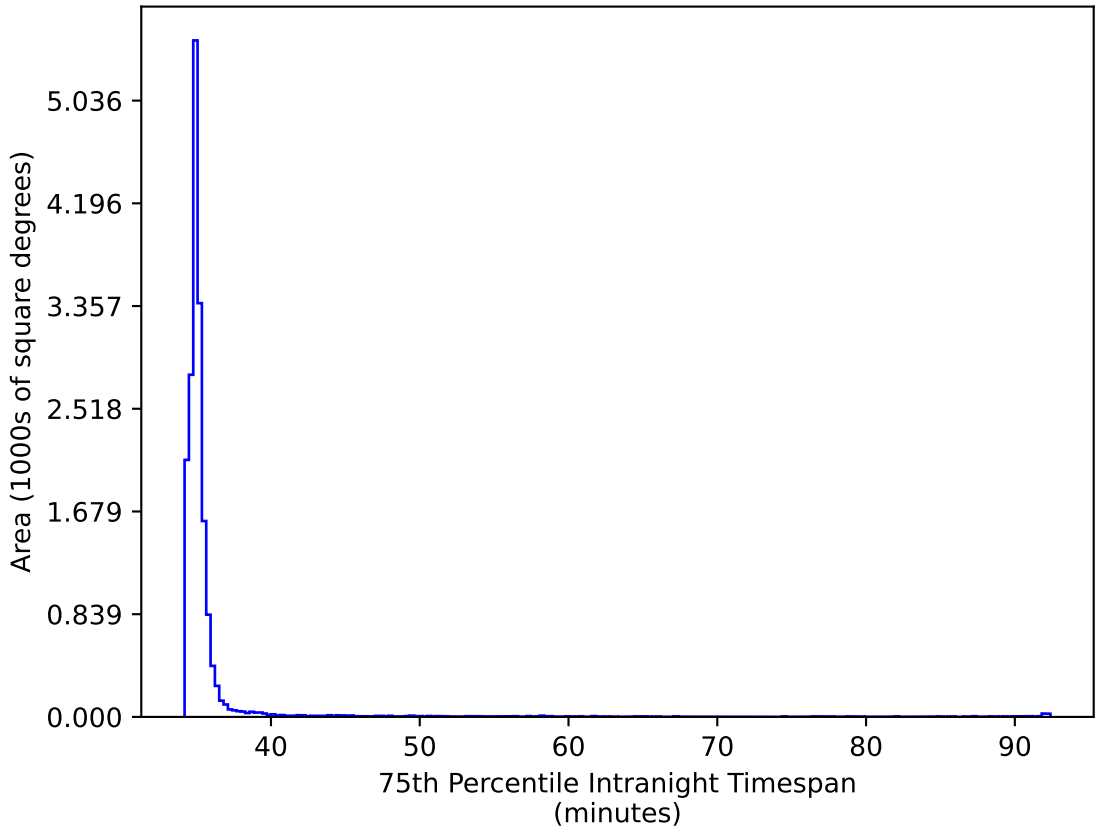
too_elab_heavy_r32_d2_ugrizy_v3.4_10yrs WFD ri bands: 75th Percentile Intranight Timespan
