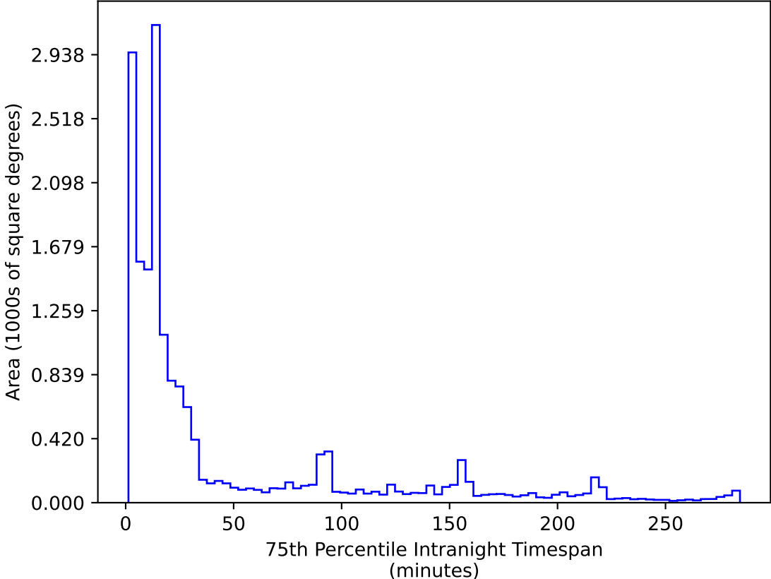
too_elab_heavy_r32_d2_ugrizy_v3.4_10yrs WFD r band: 75th Percentile Intranight Timespan
