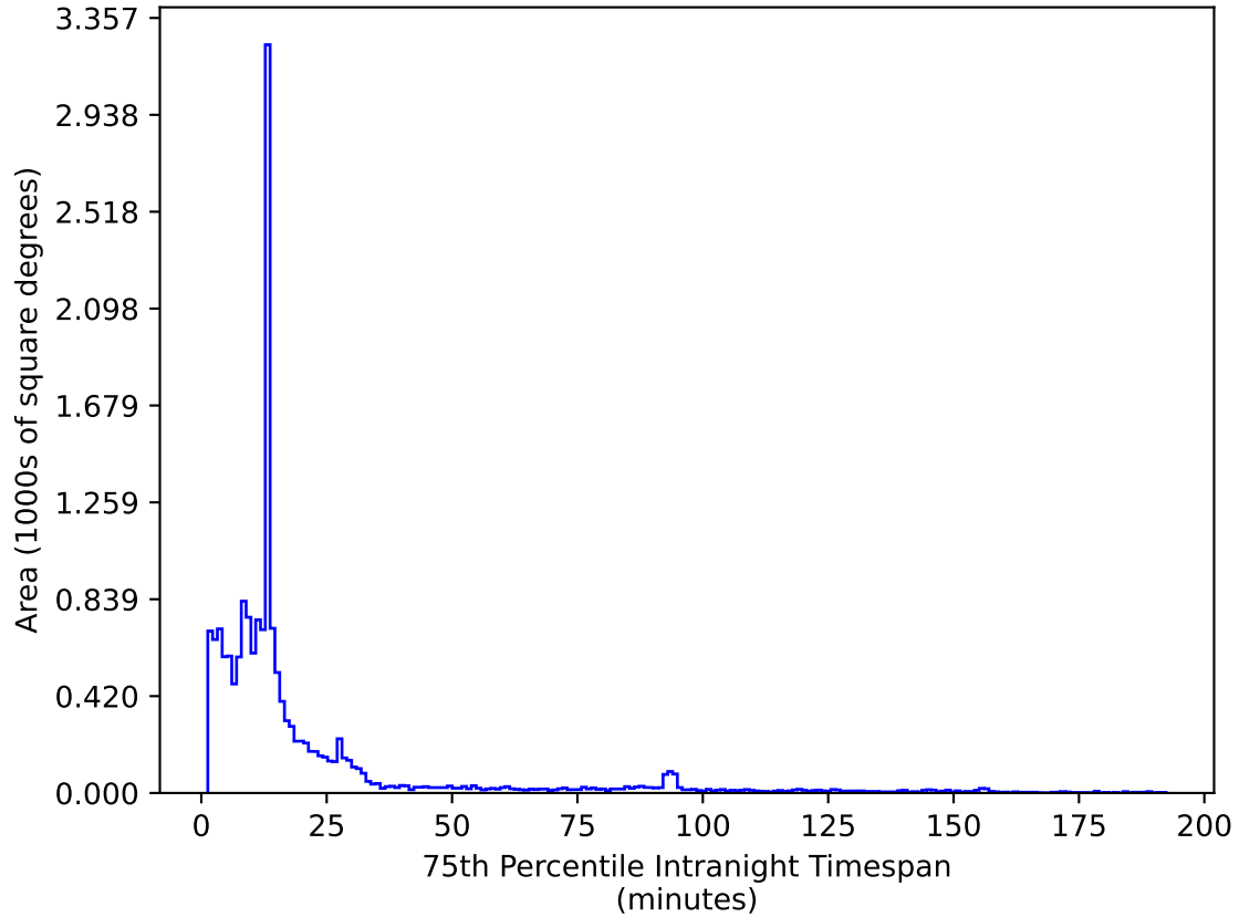
too_elab_heavy_r32_d2_ugrizy_v3.4_10yrs WFD i band: 75th Percentile Intranight Timespan
