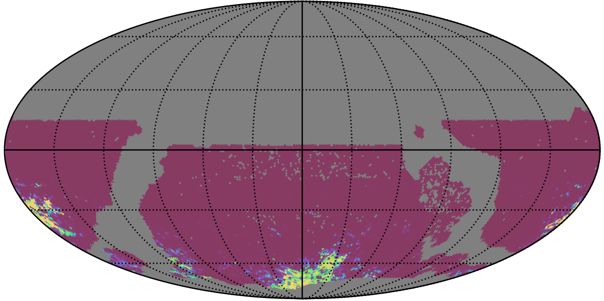
too_elab_heavy_r32_d2_ugrizy_v3.4_10yrs WFD gr bands: 75th Percentile Intranight Timespan
