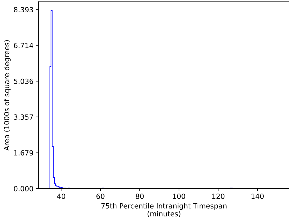
too_elab_heavy_r32_d2_ugrizy_v3.4_10yrs WFD gr bands: 75th Percentile Intranight Timespan
