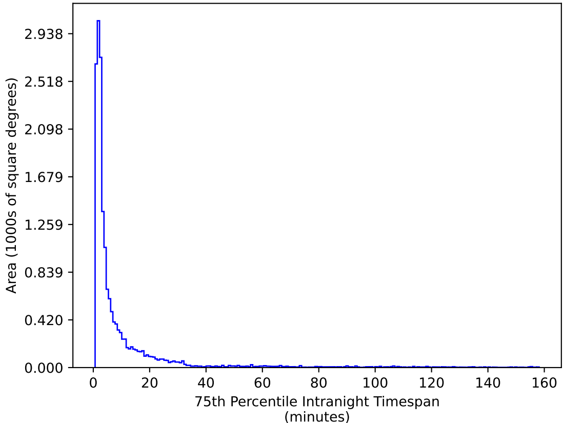
too_elab_heavy_r32_d2_ugrizy_v3.4_10yrs WFD g band: 75th Percentile Intranight Timespan
