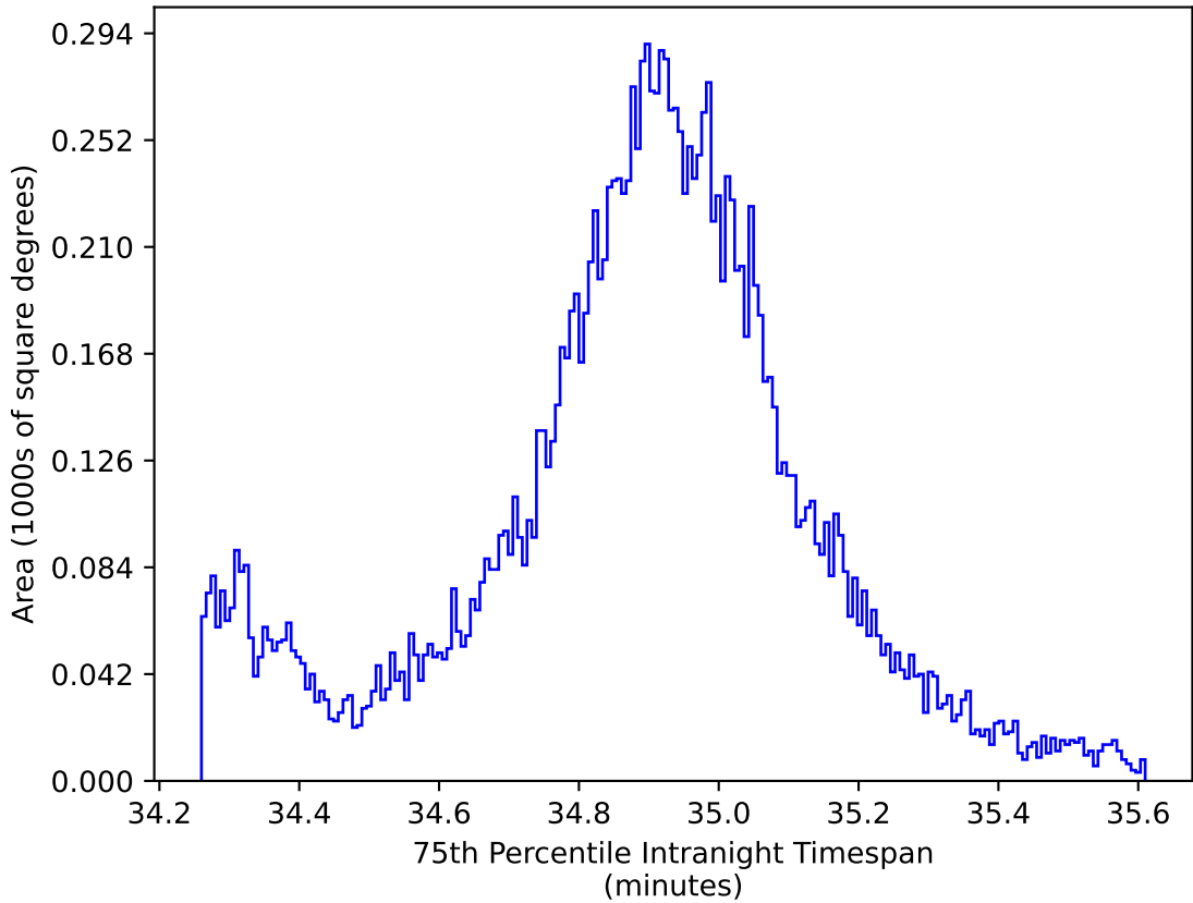
too_elab_heavy_r32_d2_ugrizy_v3.4_10yrs WFD: 75th Percentile Intranight Timespan
