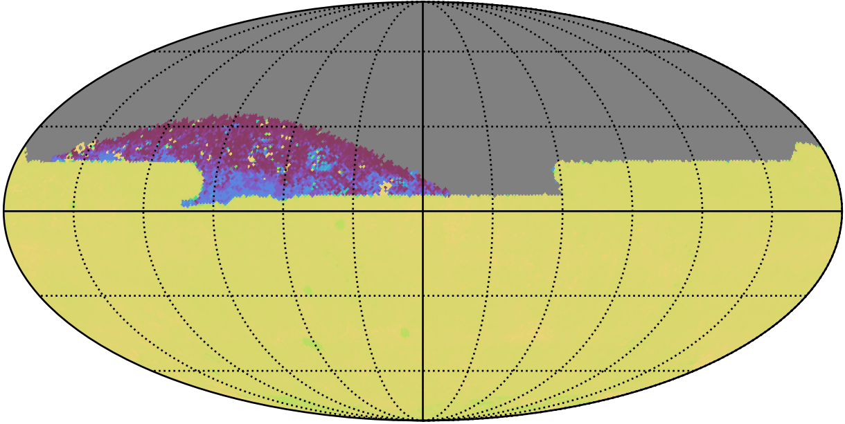
too_elab_heavy_r32_d2_ugrizy_v3.4_10yrs All sky zy bands: 75th Percentile Intranight Timespan
