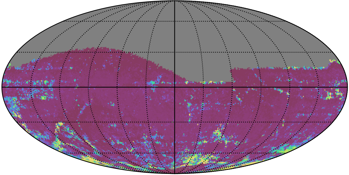
too_elab_heavy_r32_d2_ugrizy_v3.4_10yrs All sky z band: 75th Percentile Intranight Timespan
