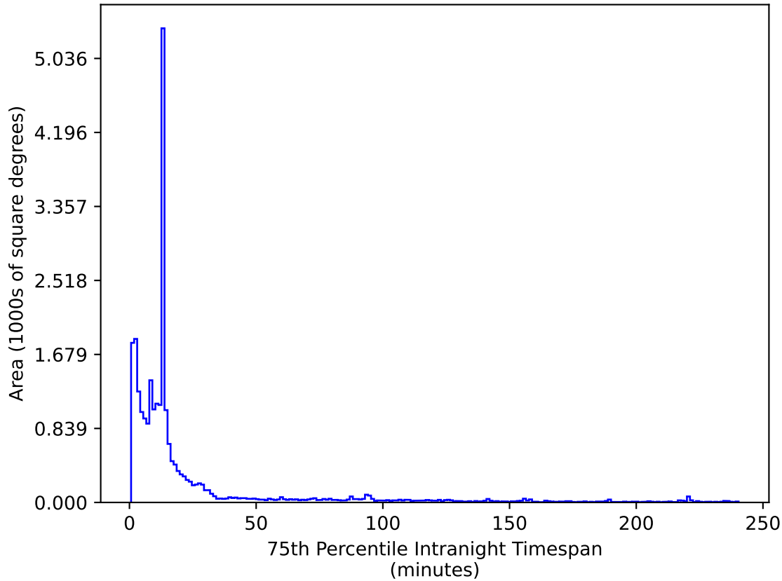
too_elab_heavy_r32_d2_ugrizy_v3.4_10yrs All sky z band: 75th Percentile Intranight Timespan
