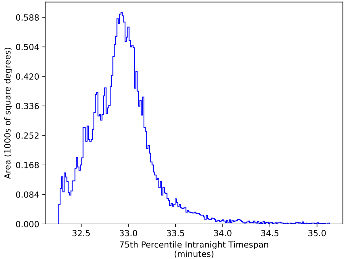
too_elab_heavy_r32_d2_ugrizy_v3.4_10yrs All sky y band: 75th Percentile Intranight Timespan
